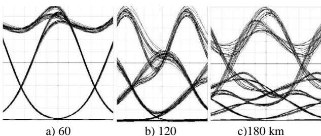
Fig.10: Post RZ encoded DWDM
