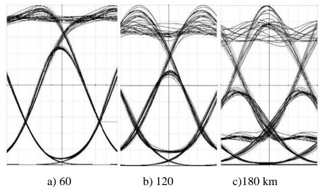
Fig.11: Pre NRZ encoded DWDM
