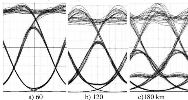
Fig.14: Pre + FBG NRZ encoded DWDM
