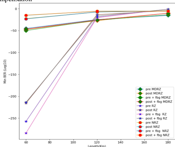
Fig.17: MIN BER Vs Transmission length with Pre and Post Compensation
