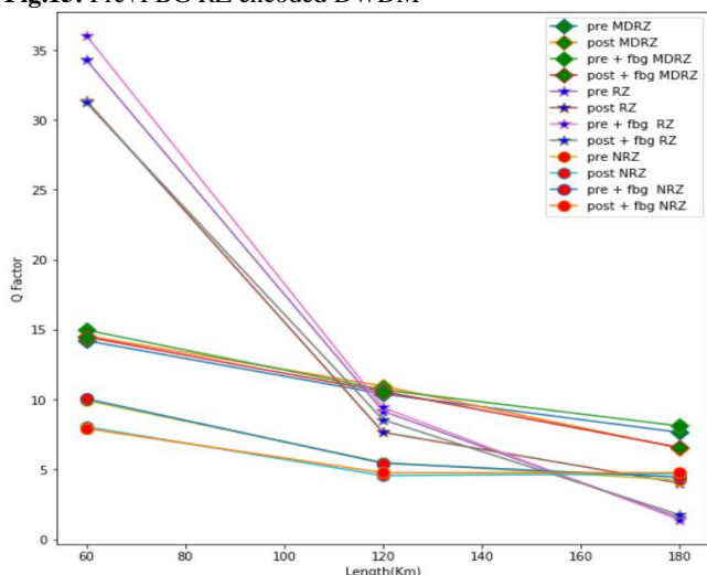
Fig.16: Q-Factor Vs Transmission length with Pre and Post Compensation
