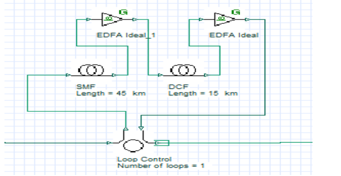
Fig. 5: Post Dispersion Compensation scheme
