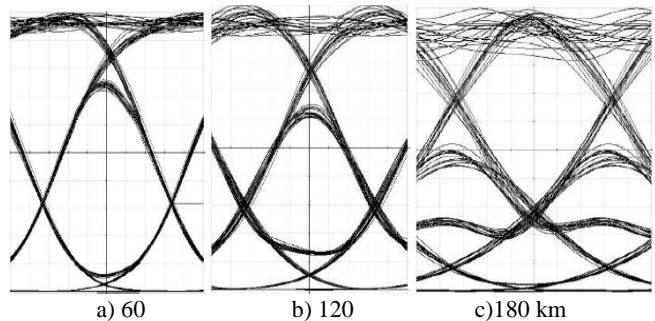
Fig.12: Post NRZ encoded DWDM
