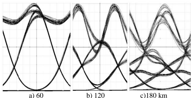
Fig.15: Pre+FBG RZ encoded DWDM
