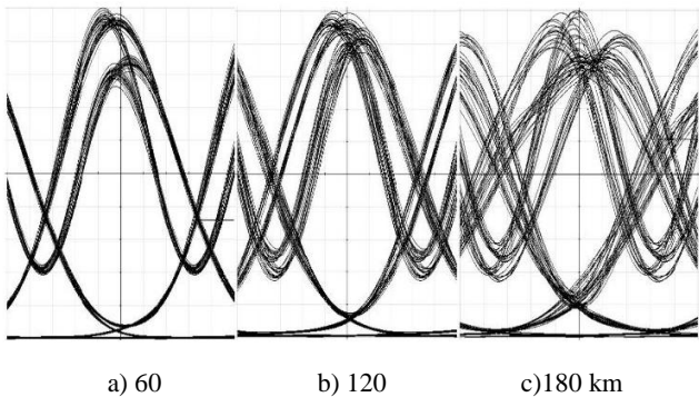
Fig. 8: Post MDRZ encoded DWDM
