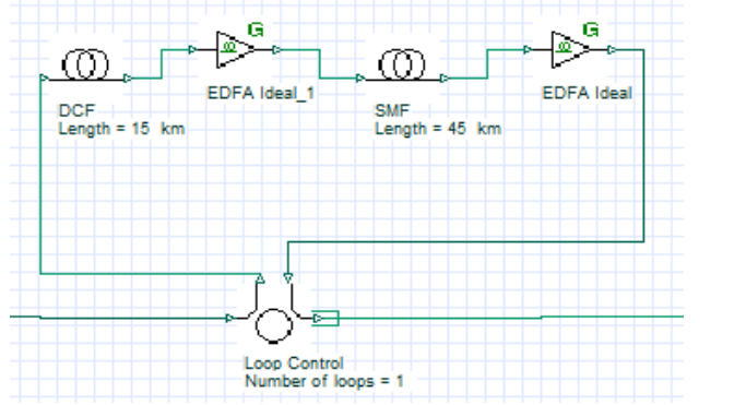
Fig. 4: Pre Dispersion Compensation scheme
