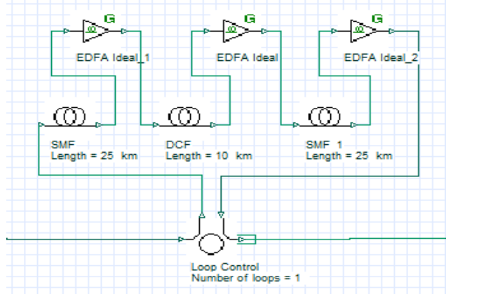
Fig. 6: Symmetrical Dispersion Compensation scheme
