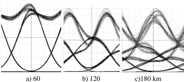
Fig.9: Pre RZ encoded DWDM
